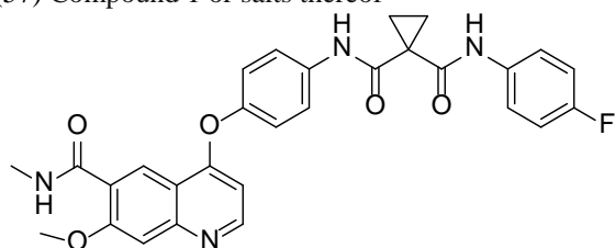
Compound 1
